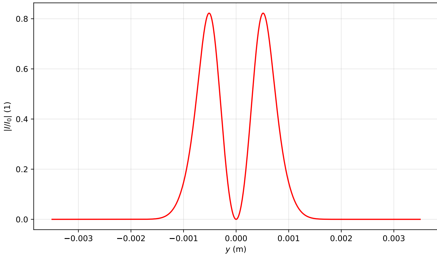
Intensity profile I(x=0, y, z=0.478)/I_0 , P_{in}=2.0P_{cr} , artificial time
